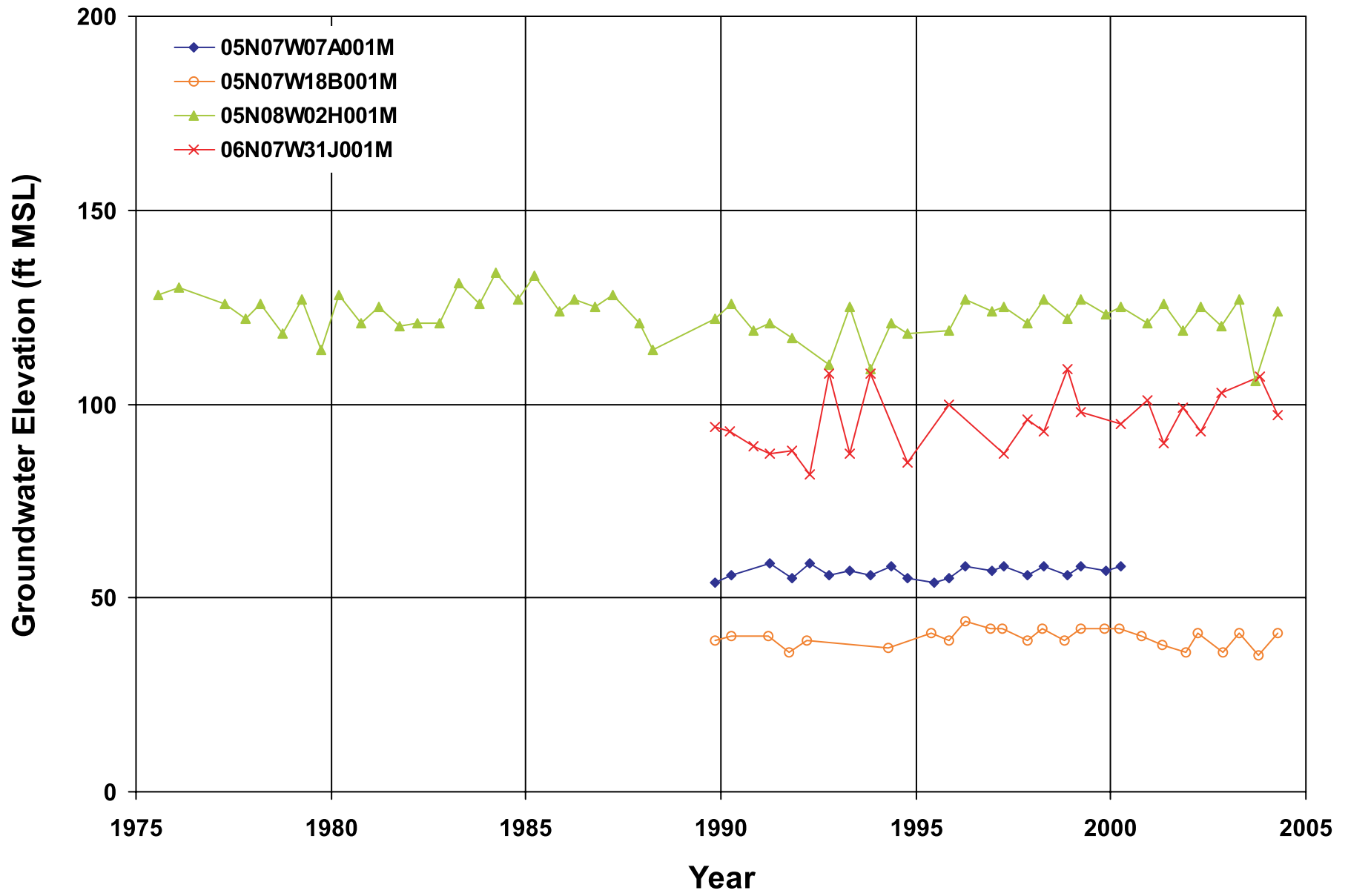
Figure 5 Hydrograph of Shallow Wells South of Groundwater Divide
